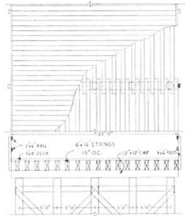
23' Thru 29' Spans
