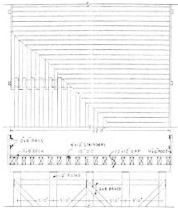
17' Thru 21' Spans
