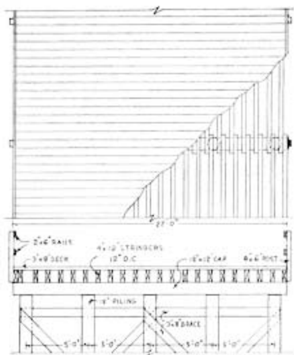
Thru 15' Spans
